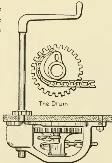
Fig. 82. Peacock Brake
